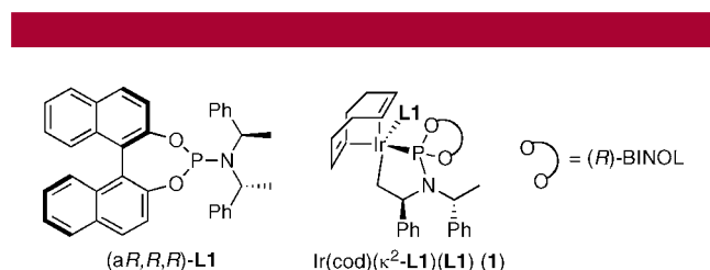
Figure 1. Structure of phosphoramidite ligand L1 and the cyclometalated, activated catalyst ( 1 ).
